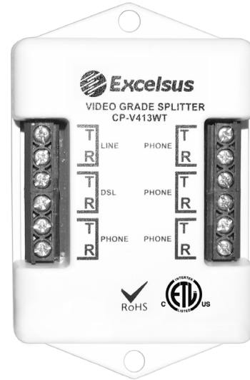
CP-V413WT VDSL2 Video-Grade CPE Splitter
