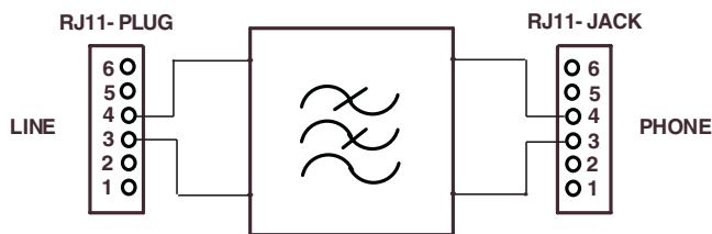
Z-301LS Block Schematic
